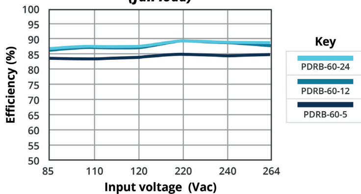
EFFICIENCY VS INPUT LOAD (full load)
