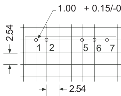
Recommended Footprint
