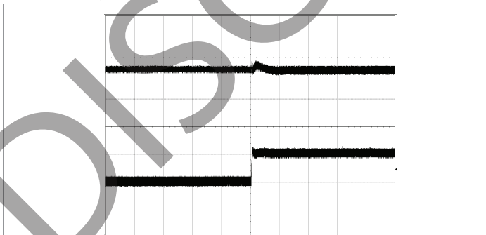
Output voltage response to input voltage transient at: T_{P1}, T_{P3} = +25^\circ\text{C}, V_i = 40\text{-}60\text{ V}, I_o = 19.5\text{ A} resistive load, C_o = 3.9\text{ mF} . Top trace: output voltage (2 V/div.). Bottom trace: input voltage (20 V/div.). Time scale: (0.5 ms/div.).
