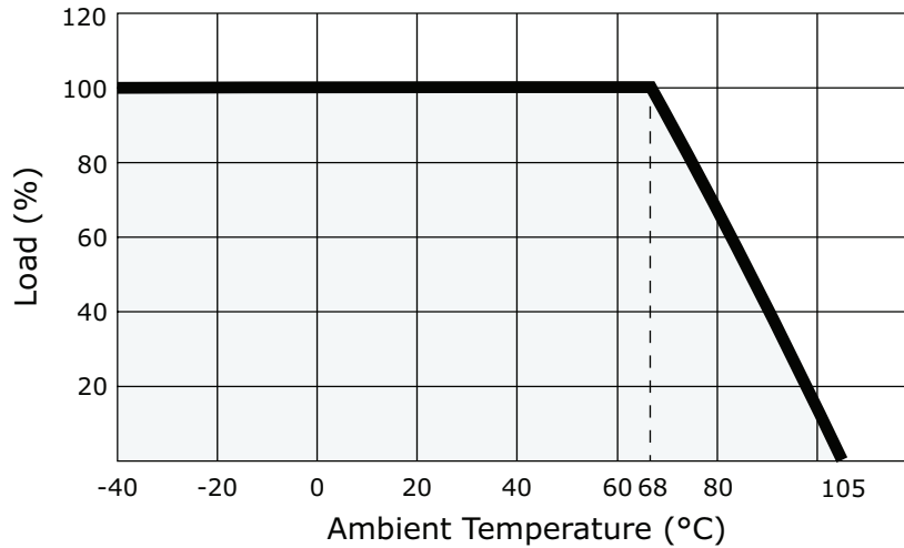
Temperature Derating Curve (Natural Convection)
