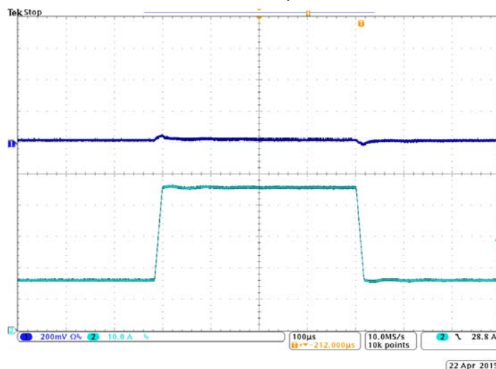
Transient Response
