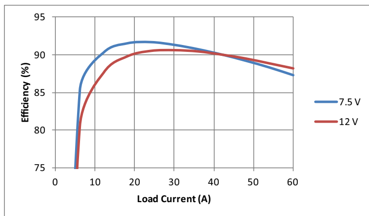
Efficiency
