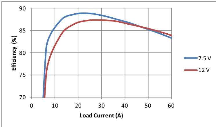
Efficiency
