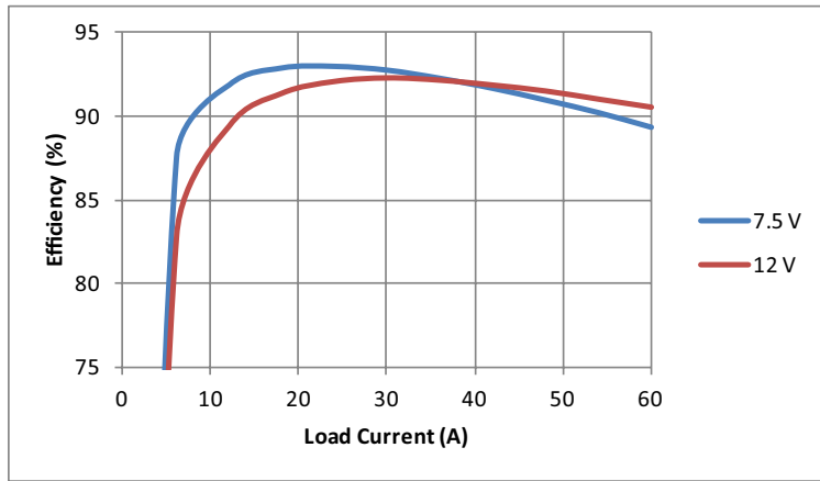
Efficiency
