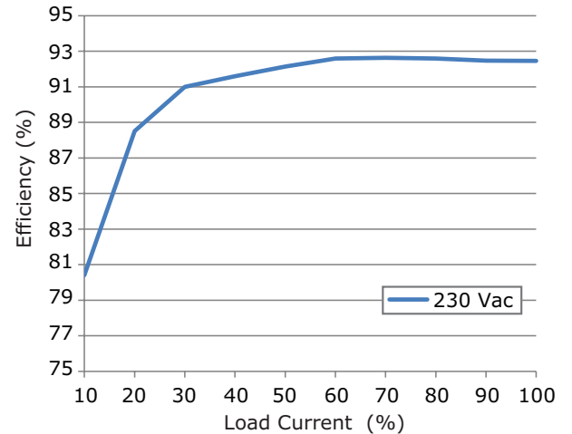
VOF-225-36 Efficiency Curve (Efficiency vs. Load Current at 230 Vac)
