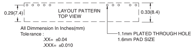
Figure 5. Recommended VPOL15A-5-SIP Footprint
