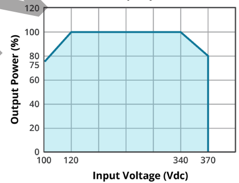
INPUT VOLTAGE DERATING CURVE (Vdc)
