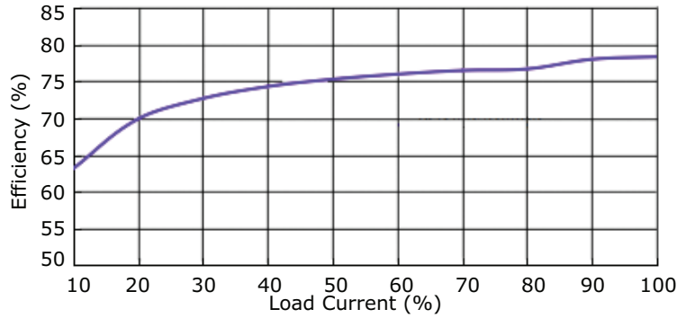
AE10-EW-S9-T Efficiency Curve Efficiency vs. Load Current
