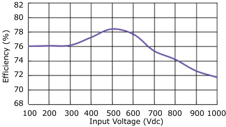
AE10-EW-S9 Efficiency Curve Efficiency vs. Input Voltage
