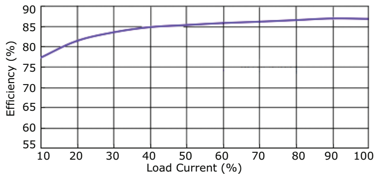
AE40-EW-S24-DIN Efficiency Curve Efficiency vs. Load Current
