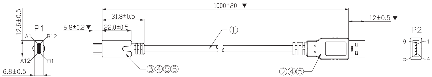
WIRING DIAGRAM
