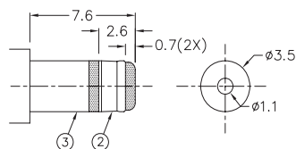
MATING PLUG
