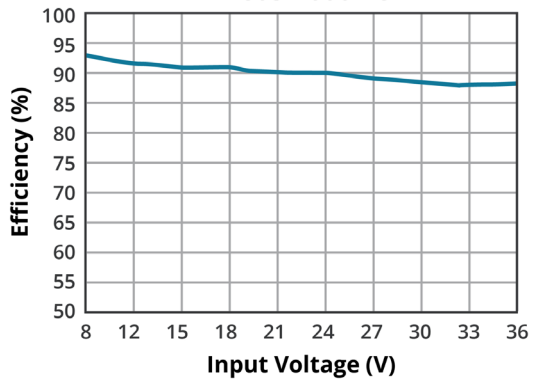
EFFICIENCY VS INPUT VOLTAGE (full load) P7805-2000R-S
