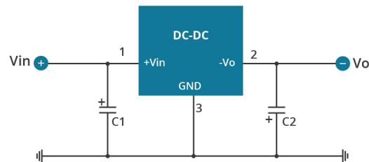
Figure 1 negative output
