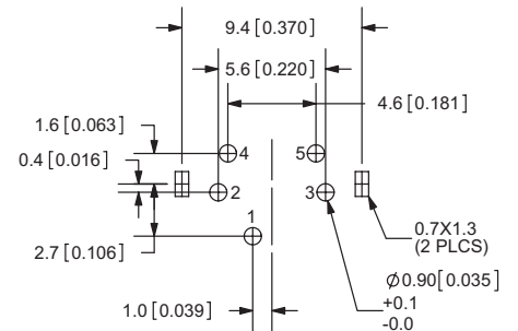
PCB LAYOUT BACK VIEW
