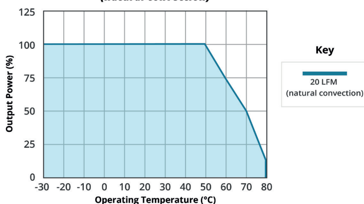
POWER DERATING CURVE (natural convection)
