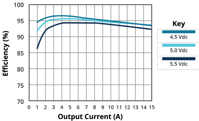
EFFICIENCY VS OUTPUT CURRENT VPOL15A-5-SMT ( V_o = 3.3 Vdc)
