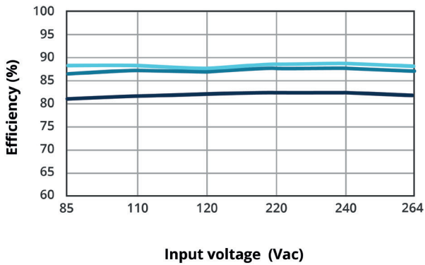
EFFICIENCY VS INPUT LOAD (full load)
