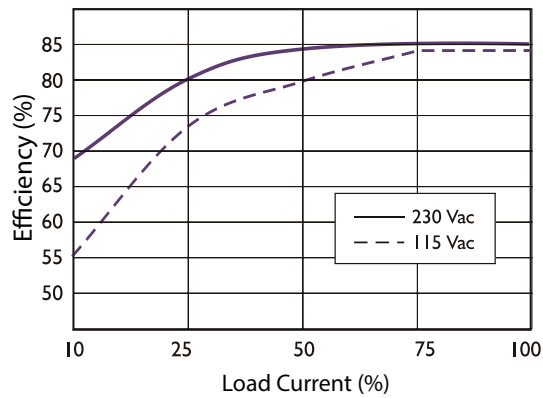
PDRC-36-24 Efficiency Curve (Efficiency vs. Load Current)
