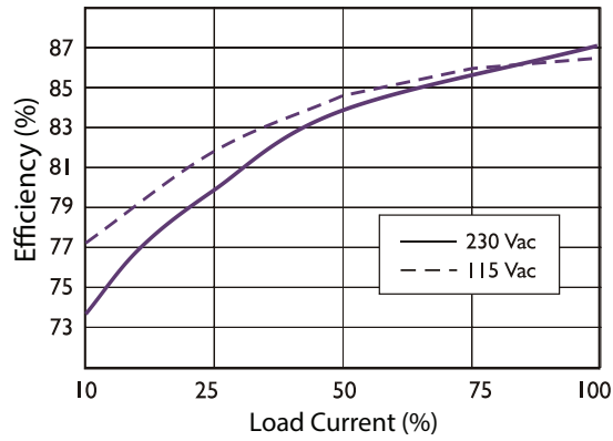
PDRC-60-24 Efficiency Curve (Efficiency vs. Load Current)
