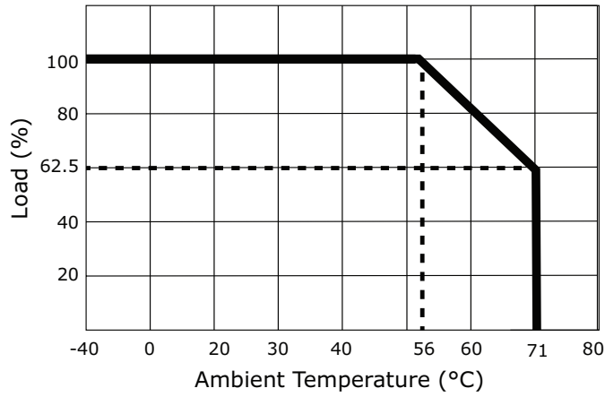
Temperature Derating Curve (Output Load vs. Ambient Temperature)
