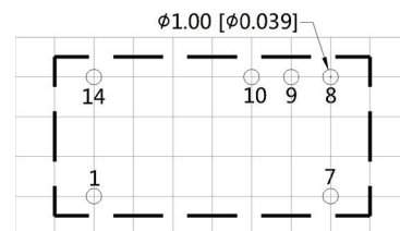
Top View PCB Layout
