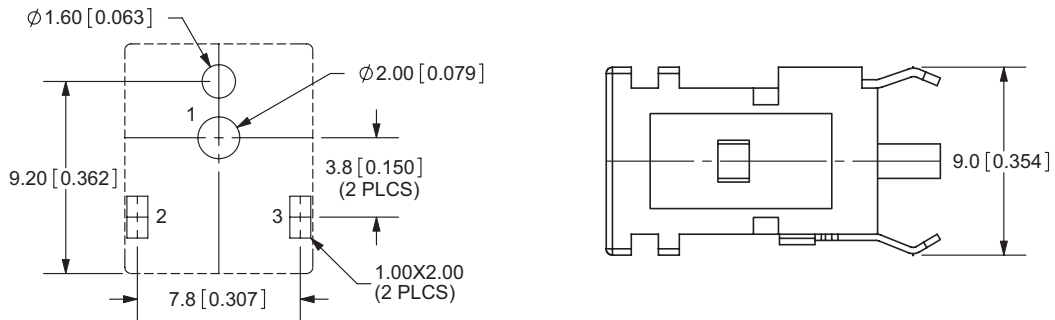
PCB LAYOUT TOP VIEW
