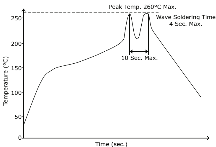
Wave Soldering Profile (DIP models)
