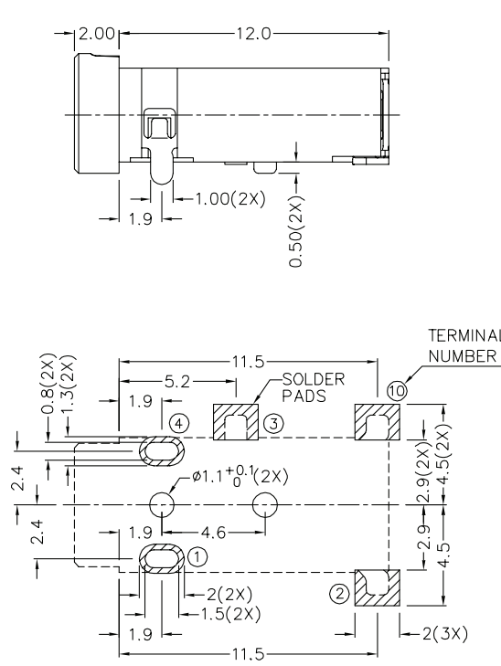
Recommended PCB Layout Top View
