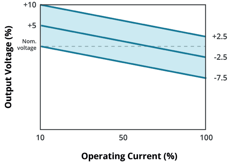
TOLERANCE ENVELOPE GRAPH
