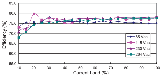
5 Vdc Output Efficiency Curve (at 25°C)
