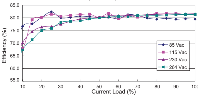
24 Vdc Output Efficiency Curve (at 25°C)
