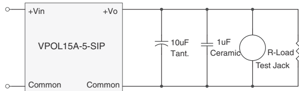
Figure 15. Output Voltage Ripple and Noise Measurement Set-Up
