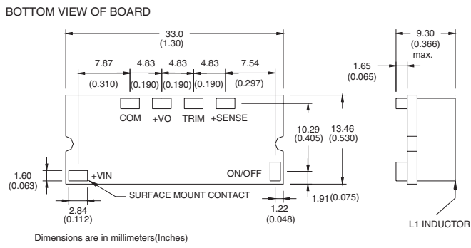
Figure 16 VPOL16A-12-SMT Mechanical Outline Diagram
