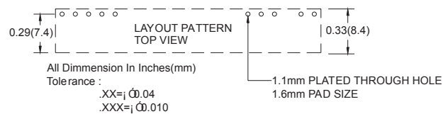
Figure 8. Recommended VPOL16A-12W-SIP Footprint
