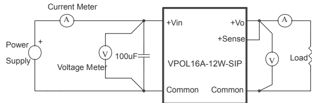
Figure 13. VPOL16A-12W-SIP Series Test Setup
