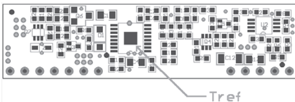
Figure 10. Temperature Measurement Location for VPOL16A-12W-SIP
