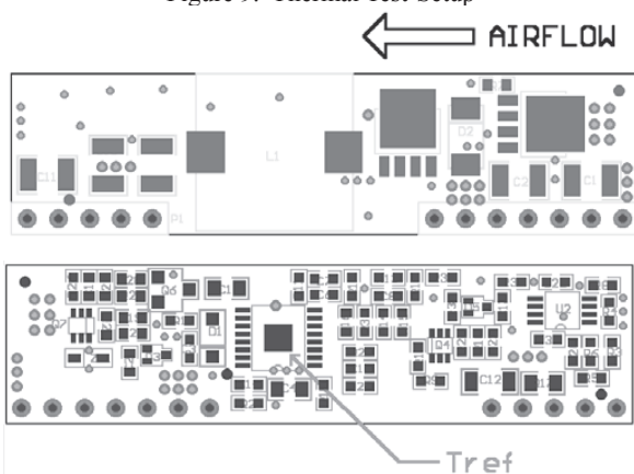
Figure 10. Temperature Measurement Location for VPOL16A-12W-SIP
