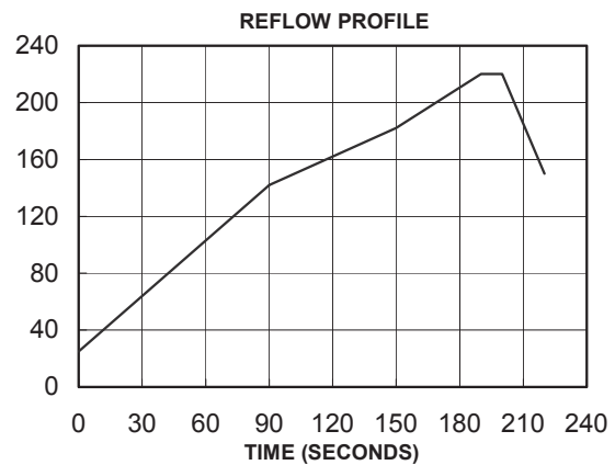
Figure 17 VPOL16A-12W-SMT Reflow Profile
