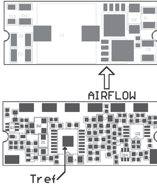
Figure 10. Temperature Measurement Location for VPOL16A-12W-SMT
