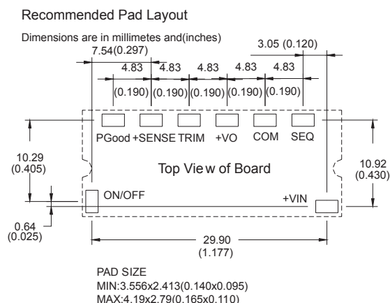
Figure 9. Recommended VPOL16A-12W-SMT Footprint
