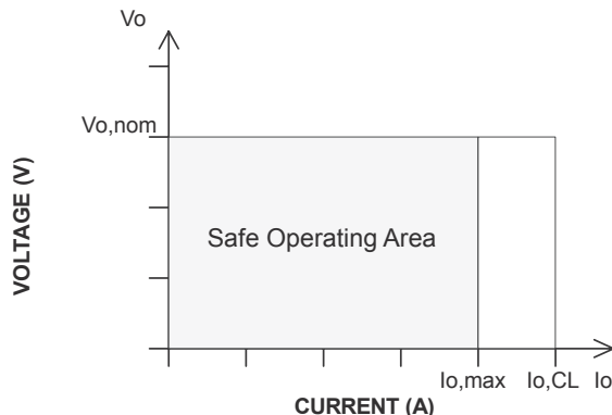
Figure 2. Maximum Output Current Safe Operating Area
