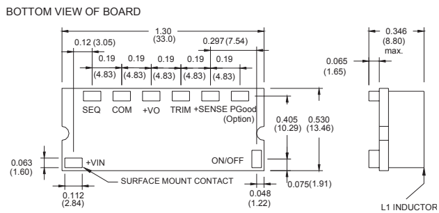
Figure 18 VPOL16A-12W-SMT Mechanical Outline Diagram
