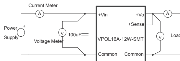
Figure 13. VPOL16A-12W-SMT Series Test Setup
