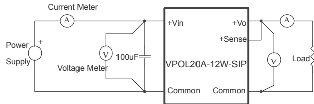
Figure 13. VPOL20A-12W-SIP Series Test Setup
