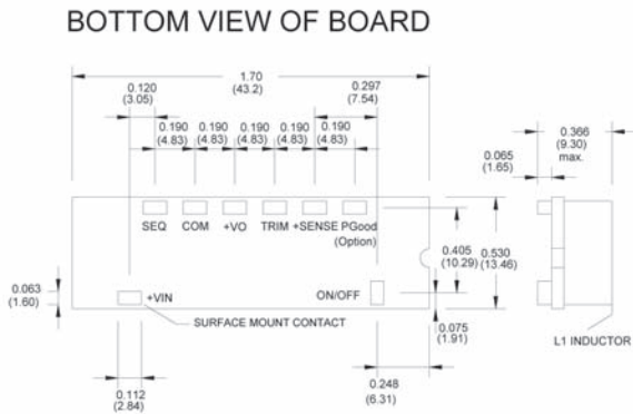
Figure 18 VPOL20A-12W-SMT Mechanical Outline Diagram
