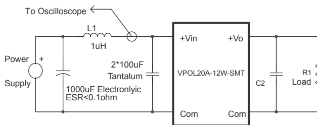
Figure 12. Input Reflected-Ripple Test Setup
