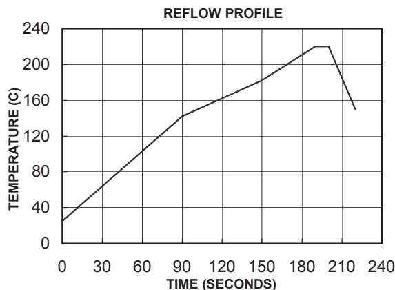
Figure 17 VPOL20A-12W-SMT Reflow Profile
