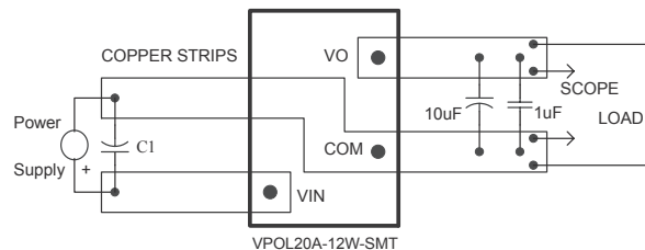
Figure 16. Output Voltage Ripple and Noise Measurement Set-Up
