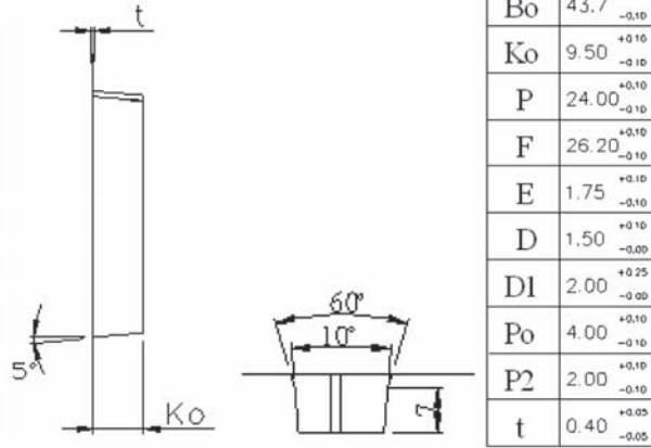
Figure 19 – VPOL20A-12W-SMT Tape and Reel Dimensions
