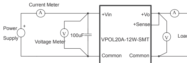
Figure 13. VPOL20A-12W-SMT Series Test Setup
